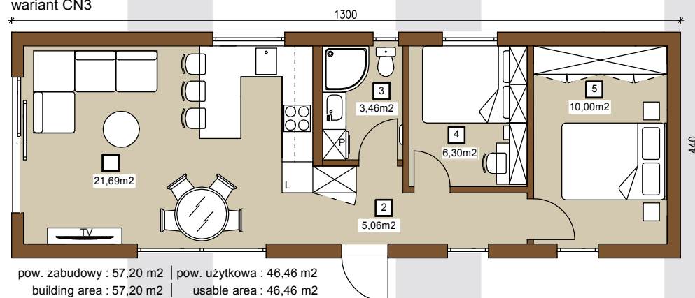
wariant CN3
